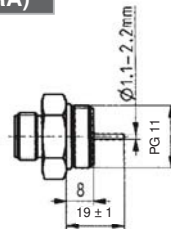
PG 11 adapter
